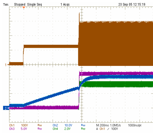
Figure 14. at 115 V AC - 60Hz
