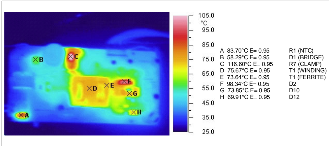
Figure 27. 115Vac-Max Load
