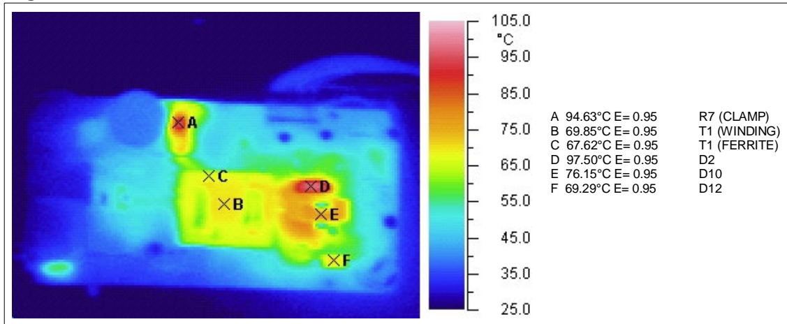
Figure 28. 230Vac-Max Load
