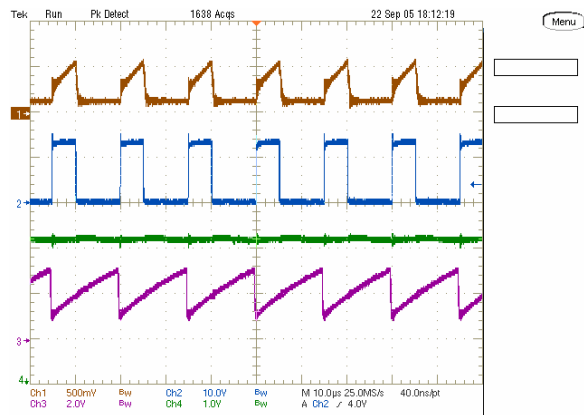
Figure 6. Vin = 115 Vrms - 60Hz
